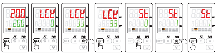
长按“SET”键3秒进入常规菜单 短按“SET”键切换为LCK菜单 短按“S”键修改为“33” 短按“SET”键进入高级菜单 短按“S”键参数闪烁 短按“R/S”或“S”键修改参数 短按“SET”键保存参数
